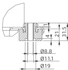
Mounting Feet
